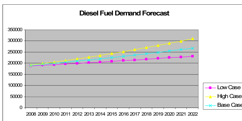
Figure 21: Diesel Fuel Demand Forecast 2008 – 2022.
