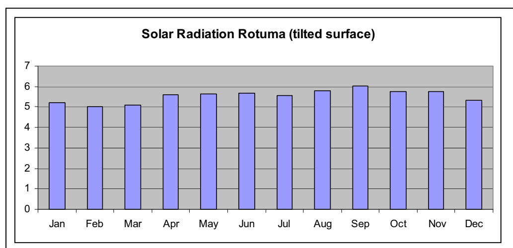
Figure 20: Solar Radiation on Rotuma (Source: NASA).
