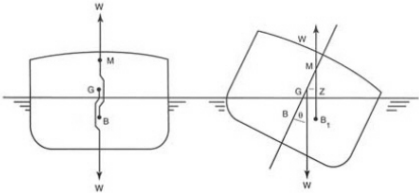
FIGURE C-1 Righting lever.
