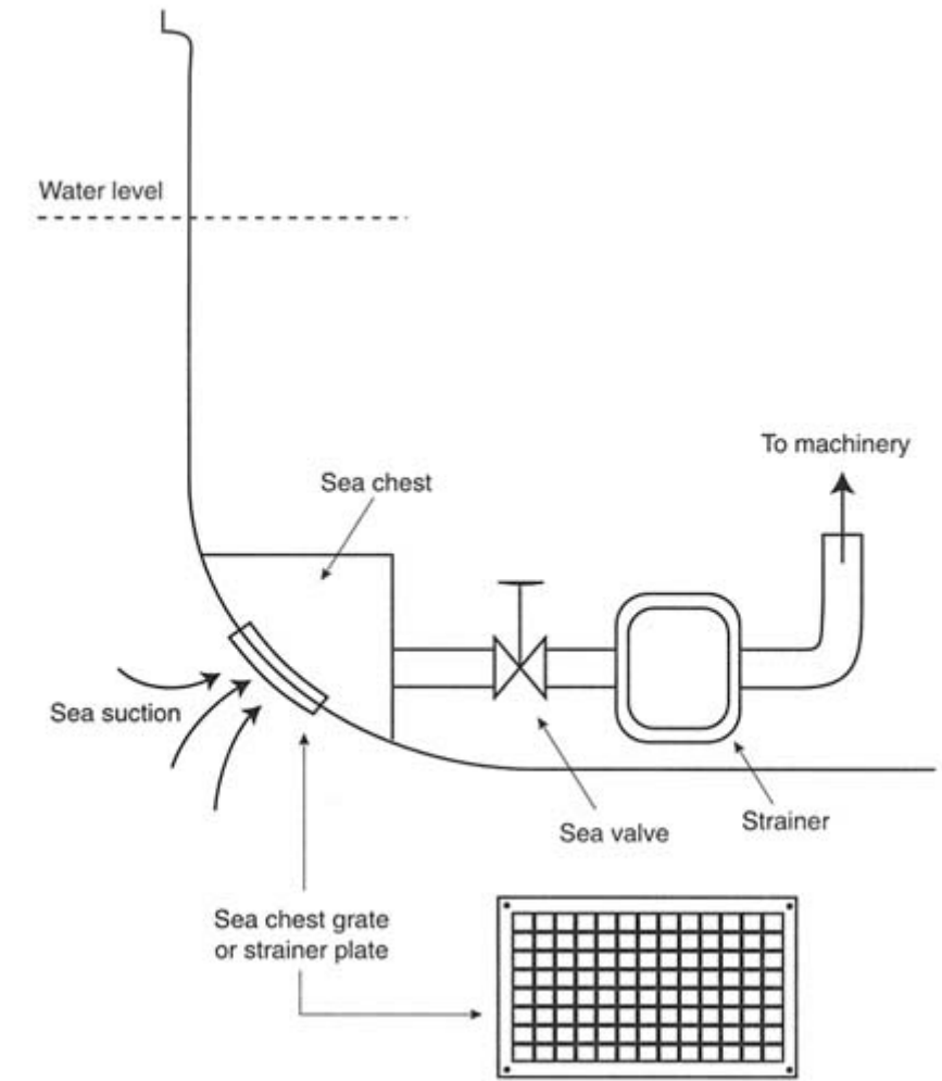
FIGURE 2-2 Typical ballast system.
