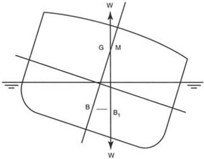
FIGURE C-2 Zero GM.
