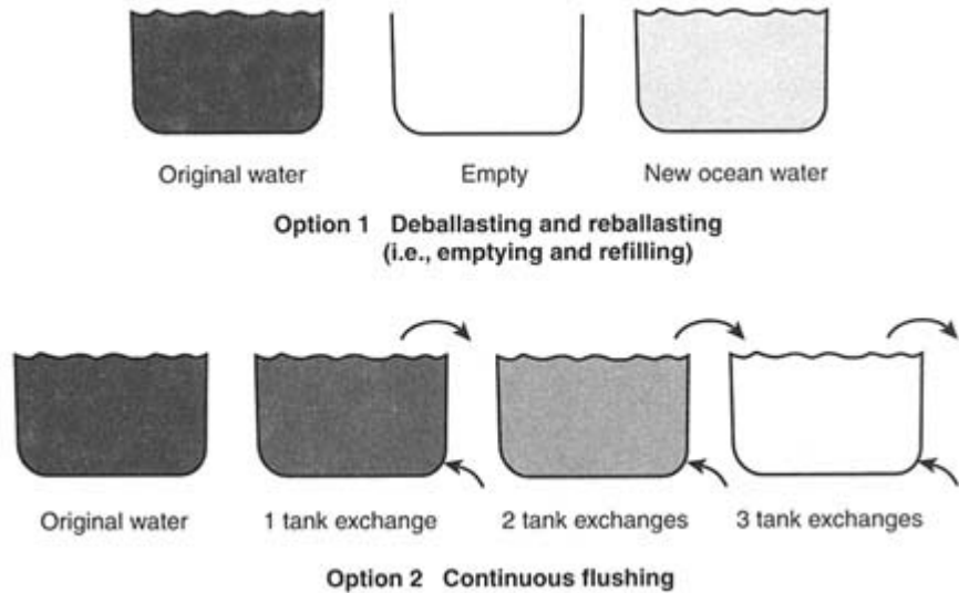
FIGURE 3-2 Basic options for changing ballast water. Note: The effectiveness of ballast water change using continuous flushing has been monitored using a dye tracer. After three tank exchanges, 95 percent of the original ballast water had been changed (AQIS, 1993). Source: Adapted from Rigby and Taylor (1994).
