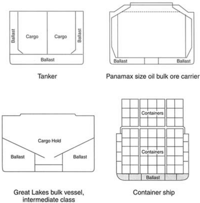
FIGURE 2-1 Typical ballast tank arrangements.
