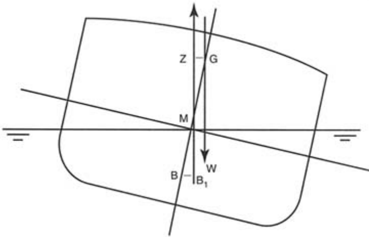
FIGURE C-4 Negative GM.
